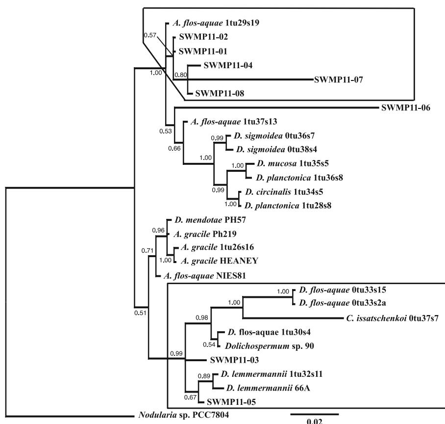
Figure 1 Phylogenetic tree for the genotypes identified from the Sacramento-San Joaquin Delta and Clear Lake (SWMP11-01 to -08).
